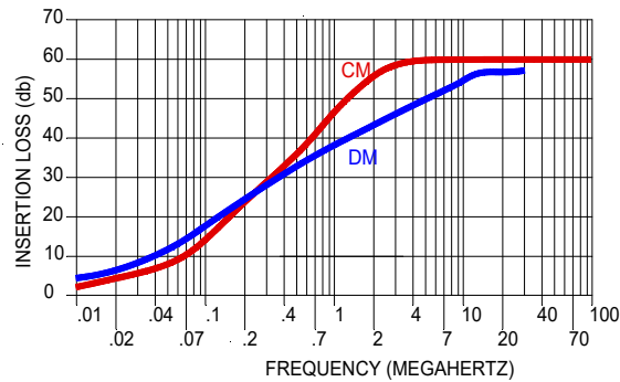
ZZ-2305-30 INSERTION LOSS - AC SECTION
