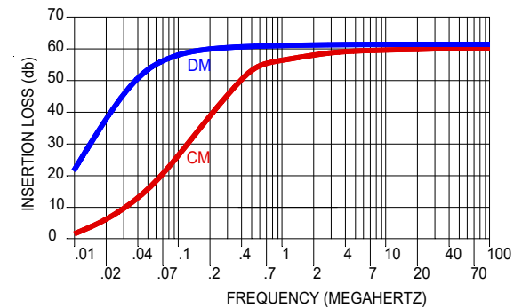
ZZ-2305-30 INSERTION LOSS - DC SECTION
