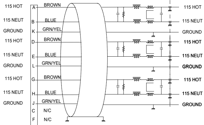
CONNECTOR D38999/20FG11PB
