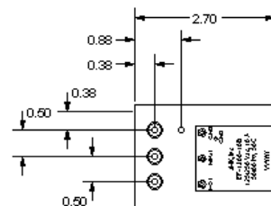
AMP P/N 172168-1 CONNECTOR WITH 170366-3 SOCKET CONTACTS
