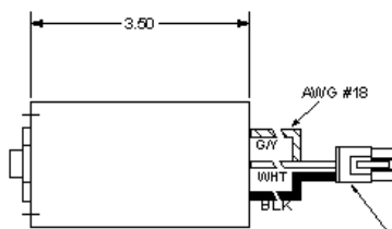
AMP P/N 172168-1 CONNECTOR WITH 170366-3 SOCKET CONTACTS
